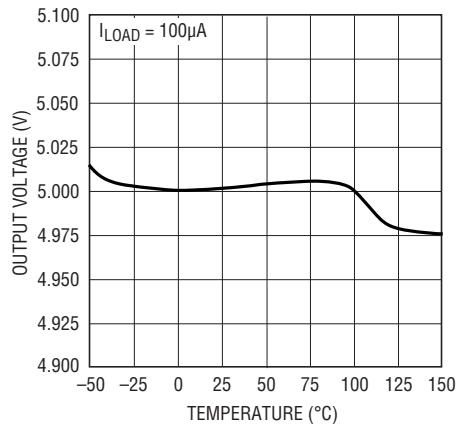
Output Voltage LT3009-5
