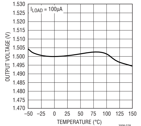
Output Voltage LT3009-1.5
