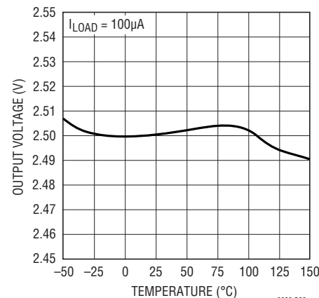
Output Voltage LT3009-2.5
