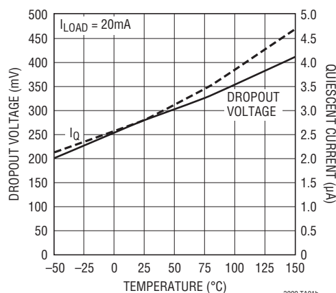
Dropout Voltage/Quiescent Current
