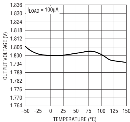
Output Voltage LT3009-1.8
